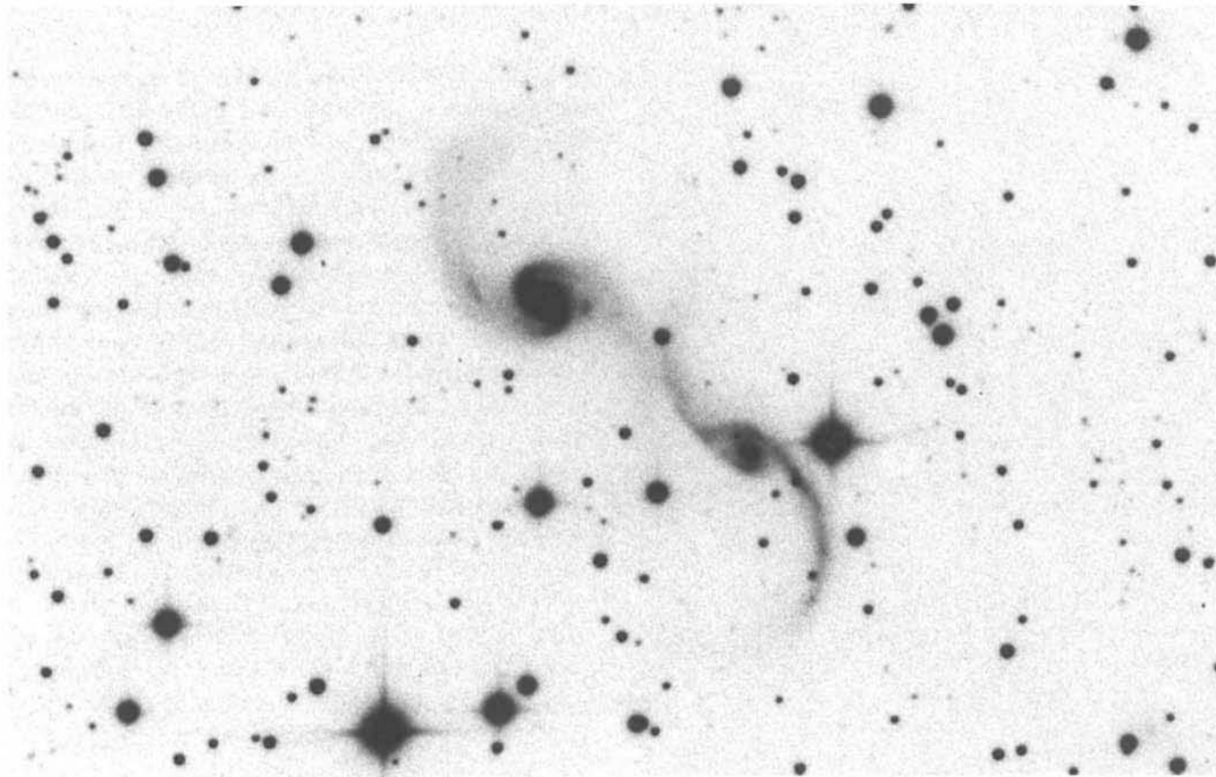
87 ESO 273-IG 04 is a distant pair (550 million light-years) with connecting arms. The projected separation of the two is 120000 light-years, somewhat less than the distance between the Milky Way Galaxy and the Large Magellanic Cloud. The larger galaxy is of the Seyfert type (see Plates 31 and 119) and has a bright nucleus.
