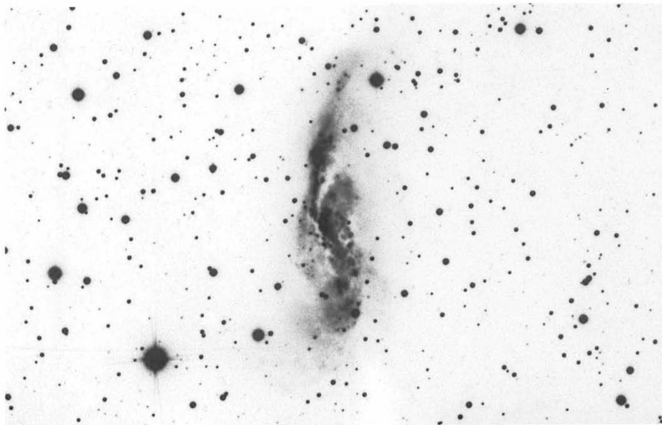
88 IC 2554 is a very disturbed pair of galaxies with a large number of emission nebulae, indicating high activity of star formation. The pair's radial velocity is moderate, 1100 km/s, which corresponds to a distance of 55 million light-years. A nearby galaxy, NGC 3136 B, is at a similar distance and may be partly responsible for the disturbances. It lies outside the field of this plate.
