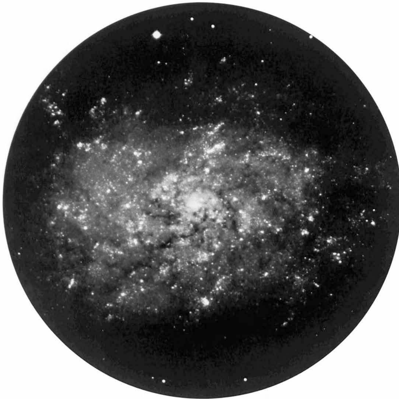
73 NGC 7793 is an Sd galaxy, and it is a splendid representative of its class. It has a small central region and a chaotic spiral pattern. The im-
