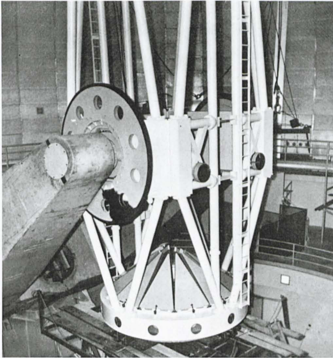
The Lick 3-m telescope when its mounting was virtually complete, in November 1954. The lower part of the telescope tube is shown, hanging on the declination axis at the top end of its long fork, the arms of which are about 7 metres long. The weight of the tube including the optics is about 40 tons (whereas the estimated weight for the ESO 3.6-m tube and optics was about 60 tons).
