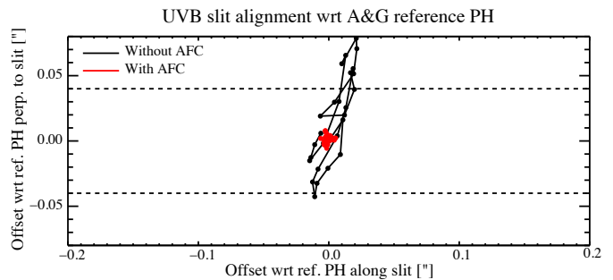
Fig. 11. Alignment of the UVB arm 0.5'' pinhole with respect to the focal plane reference pinhole with (red) and without the flexure compensation (black) through a full rotation of X-shooter at a zenith distance of 60°. The AFC allows to maintain the alignment to \sim 0.01'' , well within specification of 1/10th of the narrowest slit width.
