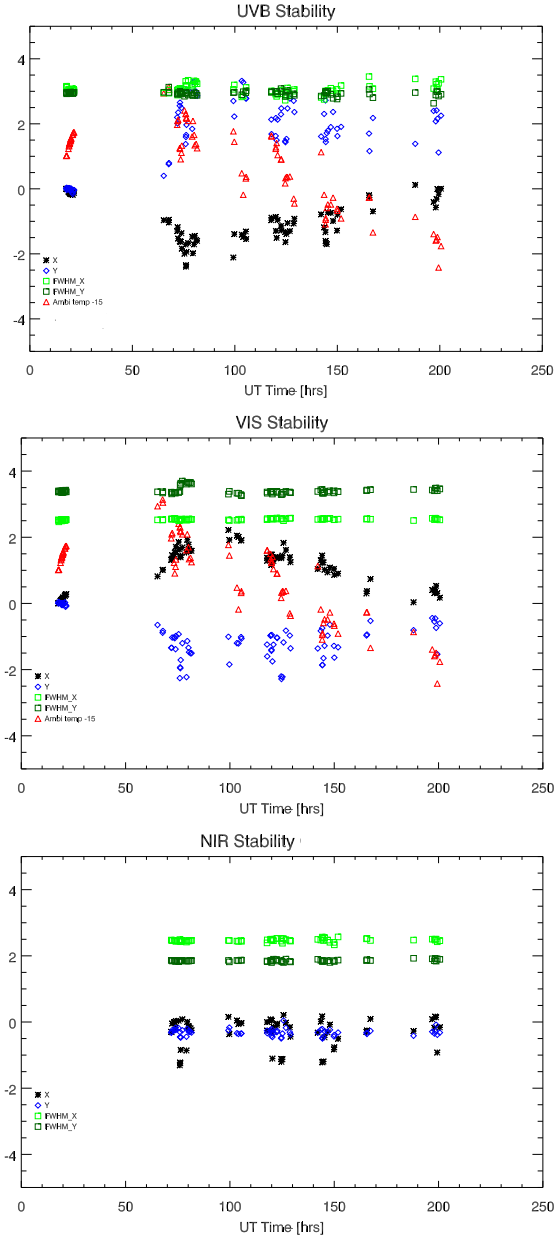
Fig. 12. Stability of the UVB (top), VIS (center) and NIR (bottom) spectrographs over 6 consecutive nights as measured during the third commissioning run. The dark and light green points show the FWHM in X and Y of a 0.5'' pinhole, the black and blue points show the X and Y position of a reference calibration line with respect to its position measured at zenith on the first day and the red points show the ambient temperature (for UVB and VIS only since it is irrelevant for the temperature controlled NIR arm).
