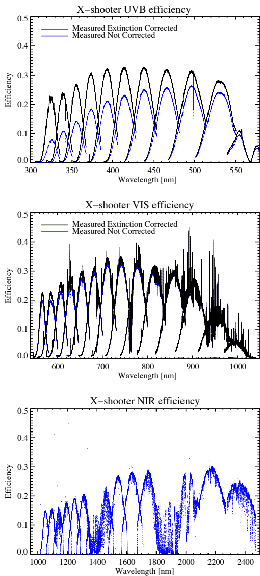
Fig. 8. The overall throughput of X-shooter, including telescope, as measured during the last commissioning run in september 2009 using spectro-photometric standard BD+17 4708. Blue curves represent raw measurements and black curves show the efficiency corrected for atmospheric extinction (UVB and VIS only).
