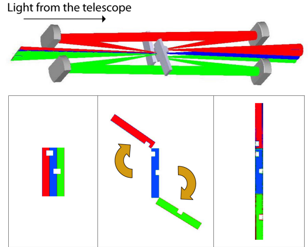
Fig. 3. Top: view of the effect of the IFU. The central field is directly transmitted to form the central slitlet (blue) while each lateral field (in red and green) is reflected toward a pair of spherical mirrors, and re-aligned at the end of the central slice to form the exit slit. Bottom: The field before (left) and after the IFU (right). The IFU acts such that the lateral fields are rotated. The two white slots are not real gaps but just guides to help visualize the top and the bottom of each slice in the drawing.
