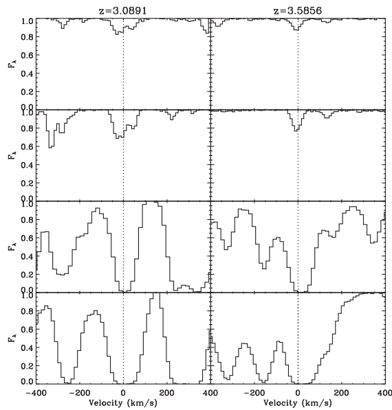
Fig. 15. The C IV \lambda 11548 \text{ \AA} and the C IV \lambda 11550 \text{ \AA} (top) lines of two high redshift metal systems in the line of sight to the QSO B1422+231 are shown in these normalized plots together with the corresponding Ly \alpha and Ly \beta absorptions. The data compare well with the observations of these systems with HIRES at Keck at three times the resolving power and from longer integration times published by Songaila & Cowie (1996). With the X-shooter, it was possible to observe all of these lines in parallel exposures within the blue and visual arm. The corresponding Mg II absorptions of the same systems fall in the NIR arm of the instrument.
