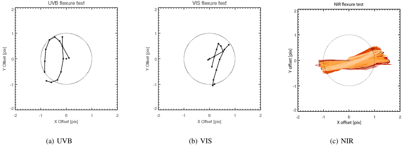
Fig. 9. Measured image position for a full rotation of the instrument at a zenith distance of 60^\circ taking as a reference (0,0) the position measured at zenith. X and Y scales are in pixels. Pixel scale is \sim 0.15''/\text{pix} for UVB and VIS, and \sim 0.2''/\text{pix} for the NIR arm. The dotted circle shows limits set by our flexure specifications: \pm 1 pixel from zenith position. In panel (a) and (b), corresponding to the UVB and the VIS arm, the curve shows the global motion of the spectral format obtained by averaging measurements obtained with five bright calibration lines. In panel (c) corresponding to the NIR arm, the track followed by many individual calibration lines during the rotation of the instrument is shown.
