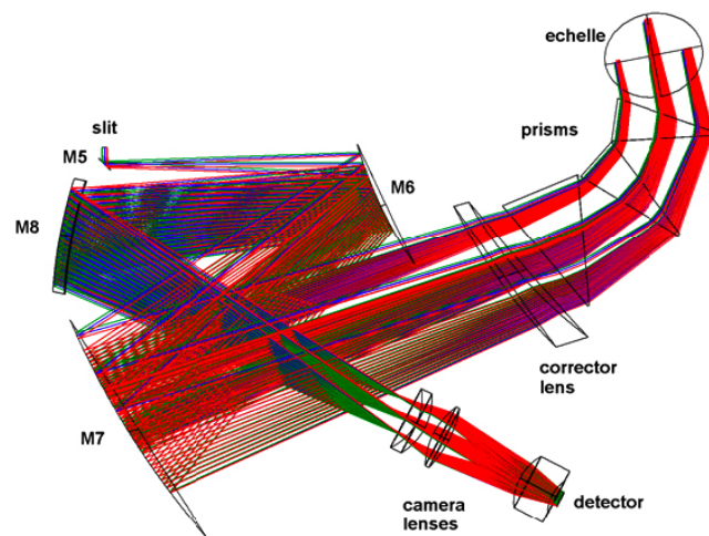
Fig. 6. The NIR spectrograph optical layout.
